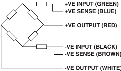
WIRING SCHEMATIC DIAGRAM (BALANCED TEMPERATURE COMPENSATION)
